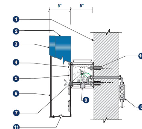
3 Section @ LED Channel Letter
