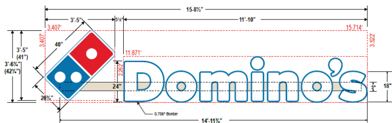
A Dom Horiz WM Channel-Raceway 24\" White
