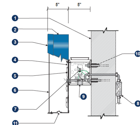
Section @ LED Channel Letter Front-Lit (Remote)
