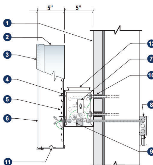
Section @ LED Channel Logo w/ Raceway Front-Lit (Remote)
