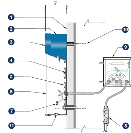
3 Section @ LED Channel Letter Front-Lit (Remote)
