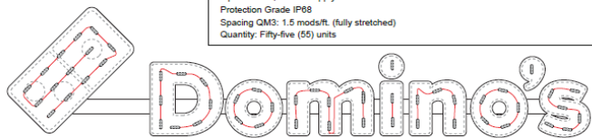
LED PATTERN SCALE: 1/2"=1'-0"
