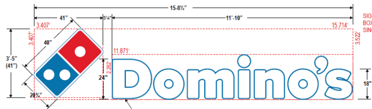
Domino's Horizontal Wordmark Channel 24" White SCALE: 1/2" = 1'-0"
